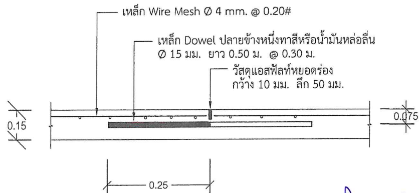
CONTRACTION JOINT
